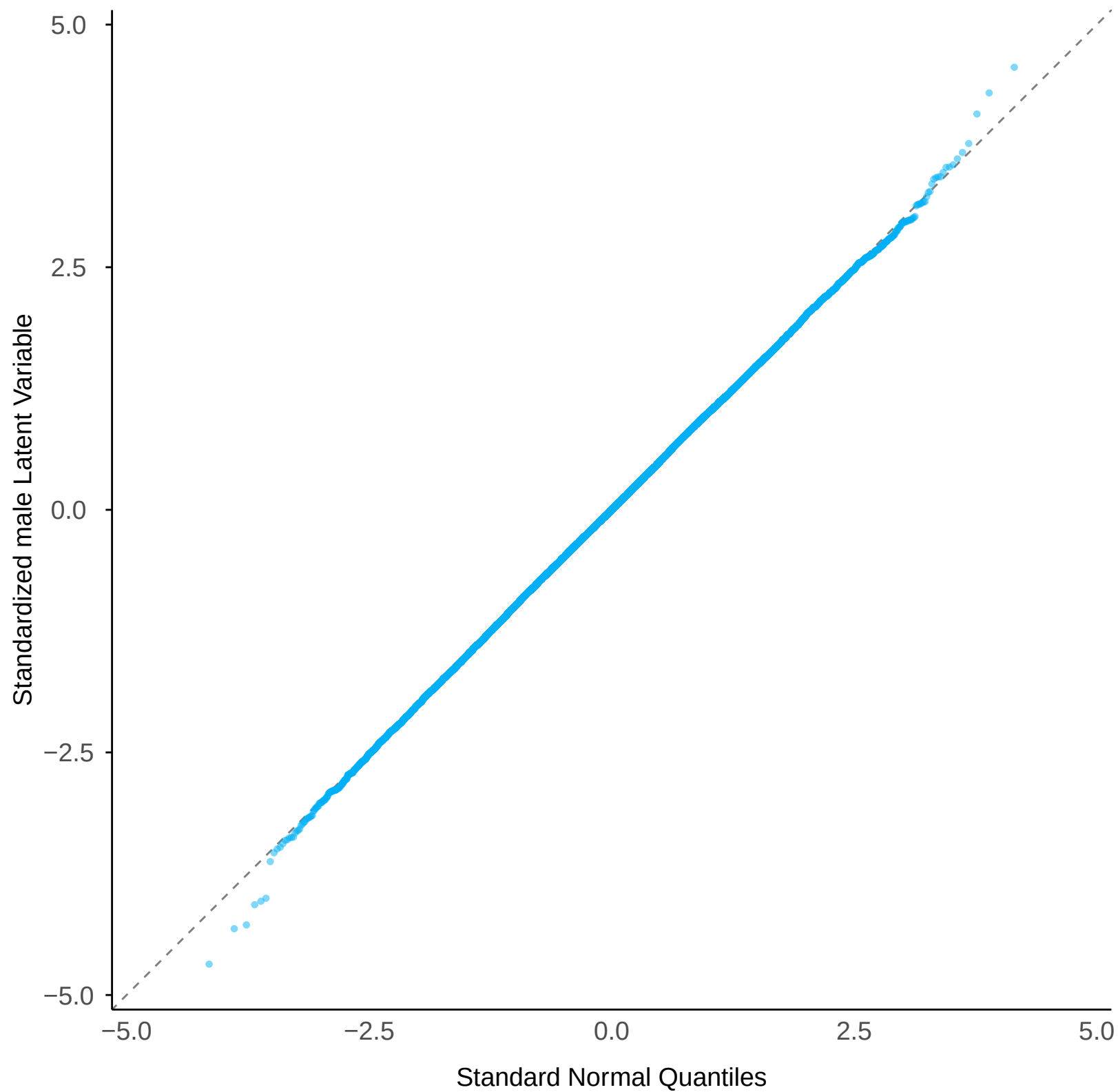
Normal Q-Q: male Latent Variable
